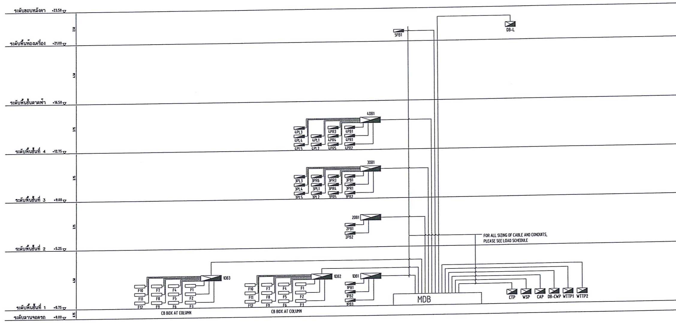
LOW DISTRIBUTION RISER DIAGRAM
